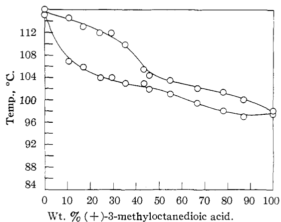
Fig. 1.—Melting point-composition diagram for the system (+)-3-methyloctanedioic acid (VII)-(-)-3-thiolactone (V).
