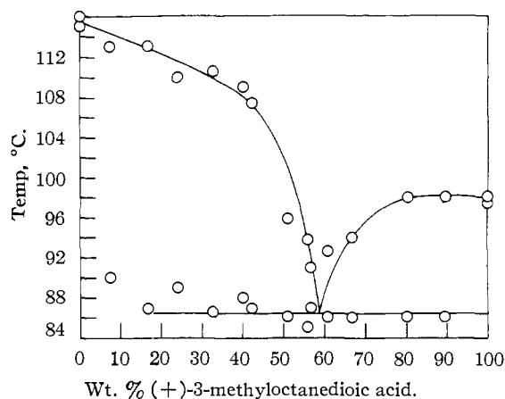
Fig. 2.—Melting point-composition diagram for the system (+)-3-methyloctanedioic acid (VII)-(+)-3-thiolactone (VI).
